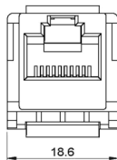
Front Aspect
